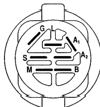
PTO SWITCH (MATING SIDE)
