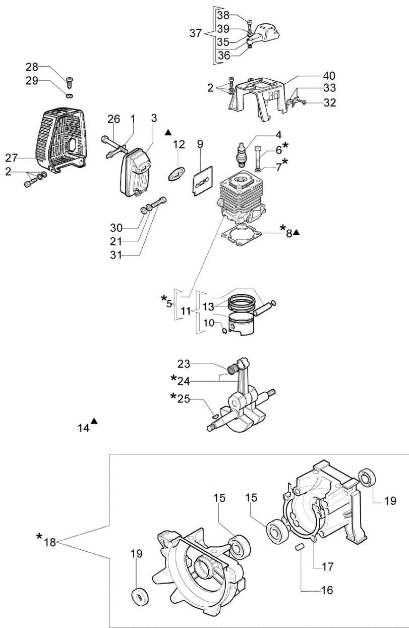
*22 Short Block
